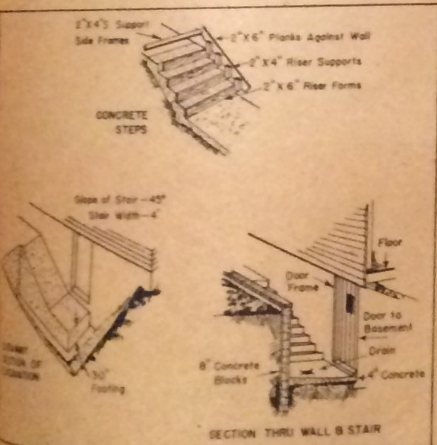
Plans for outside stairs and basement exit door, with concrete block retaining wall and cast concrete steps. Do not excavate below house footing.
