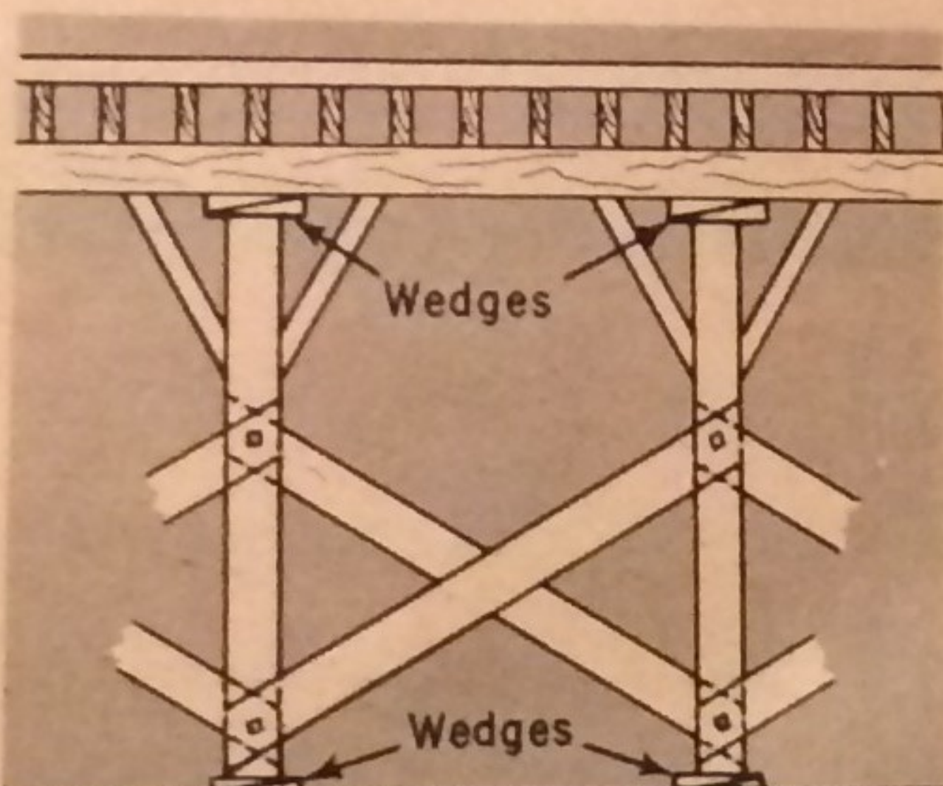
TIMBER STRUTTING FOR BASEMENT
