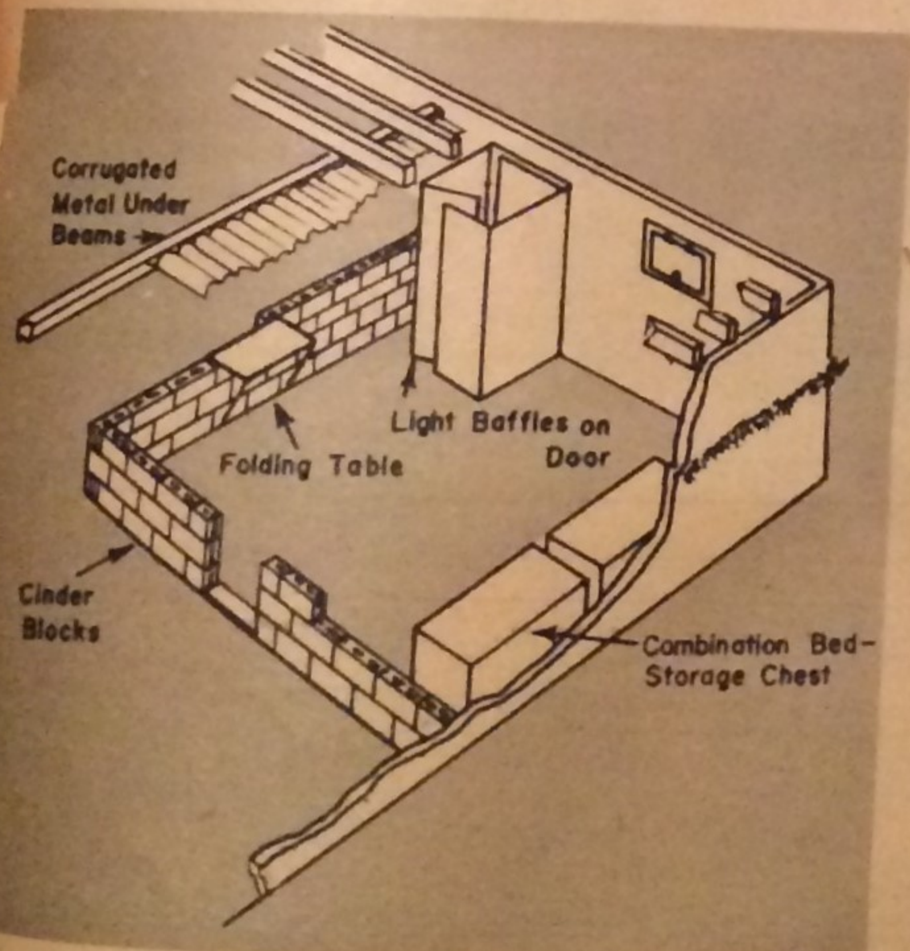
Cinder-block walls partition off section which includes outside exit protected with light baffle as protection against atomic flash.
